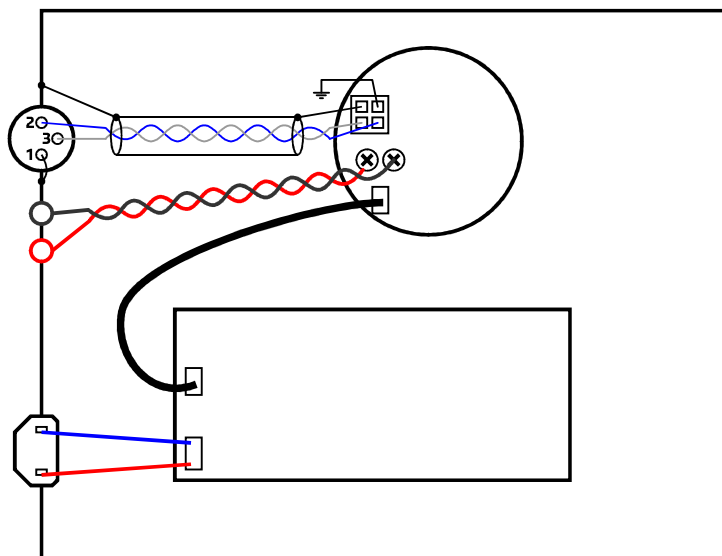
Figure 2: Preferred connection
