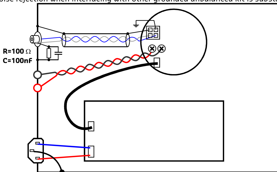
Figure 5: Solution if both mains earthing and RCA inputs are wanted
