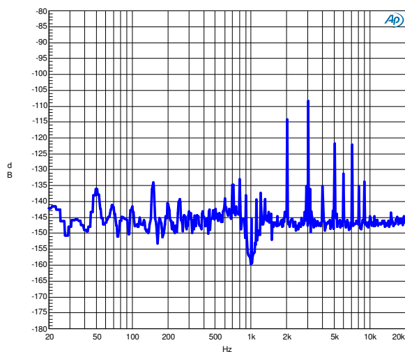
Distortion residual at 200W, 1kHz.
