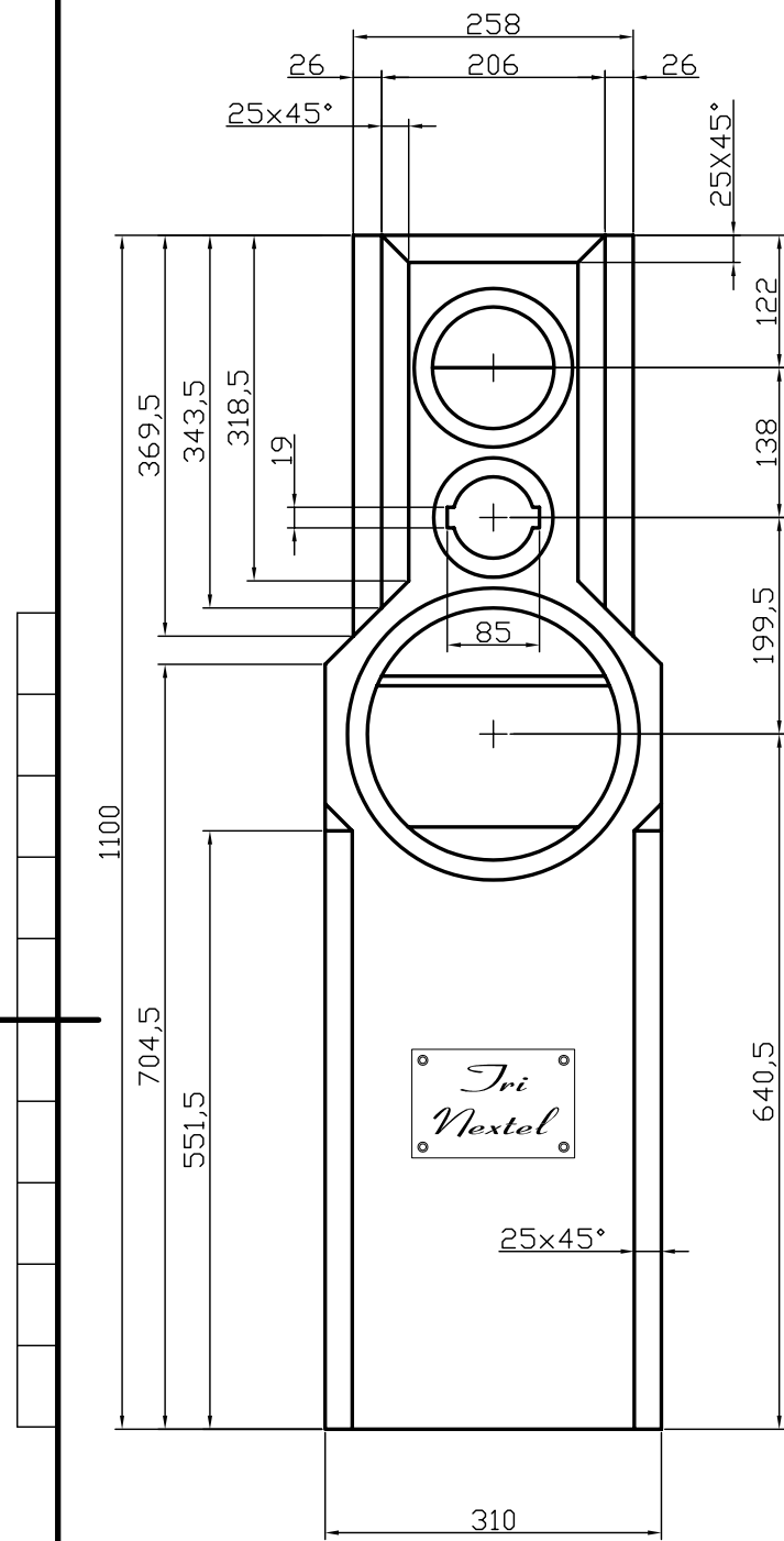
WITH BAFFLE
