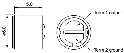
Original electret capsule
