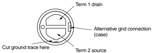
Modification to electret capsule
