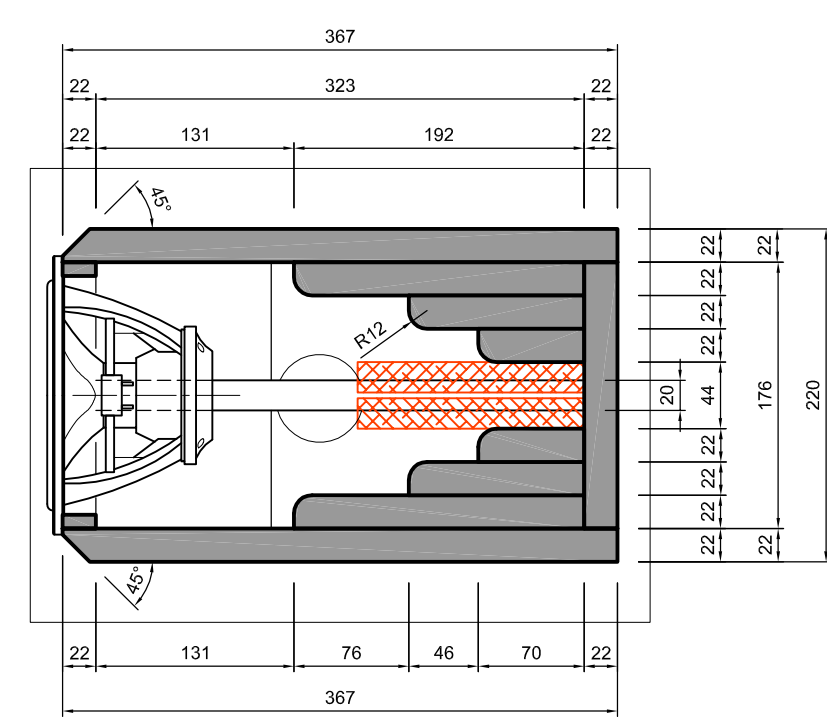
horizontal section
