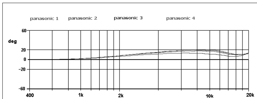
FIGURE 4: The phase response of the standard microphone.
