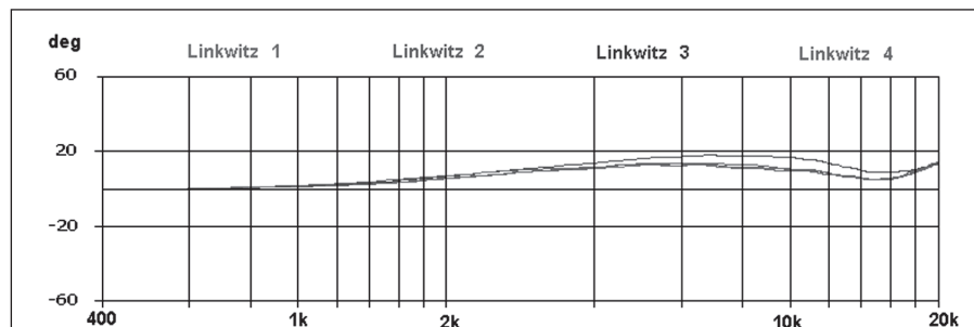
FIGURE 7: The phase response of the modified microphone.
