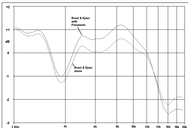
Figure 1: Two frequency responses of the same acoustic source are shown. One was taken with the B&K mike alone and the other was taken again with the B&K mike having the Panasonic mike attached on the body. The difference in the responses is due to the proximity of the Panasonic microphone.
