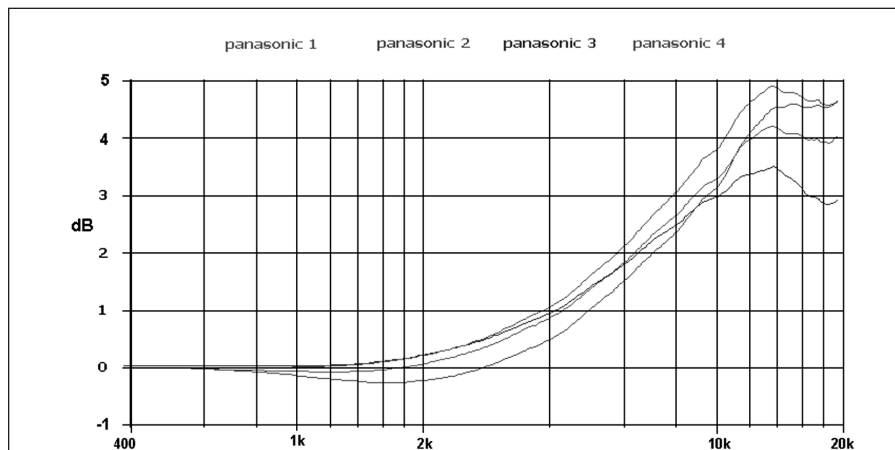
FIGURE 3: The middle- and high-frequency response of the standard microphone.
