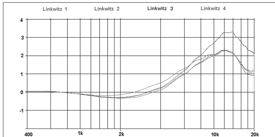
FIGURE 6: The middle- and high-frequency response of the modified microphone.
