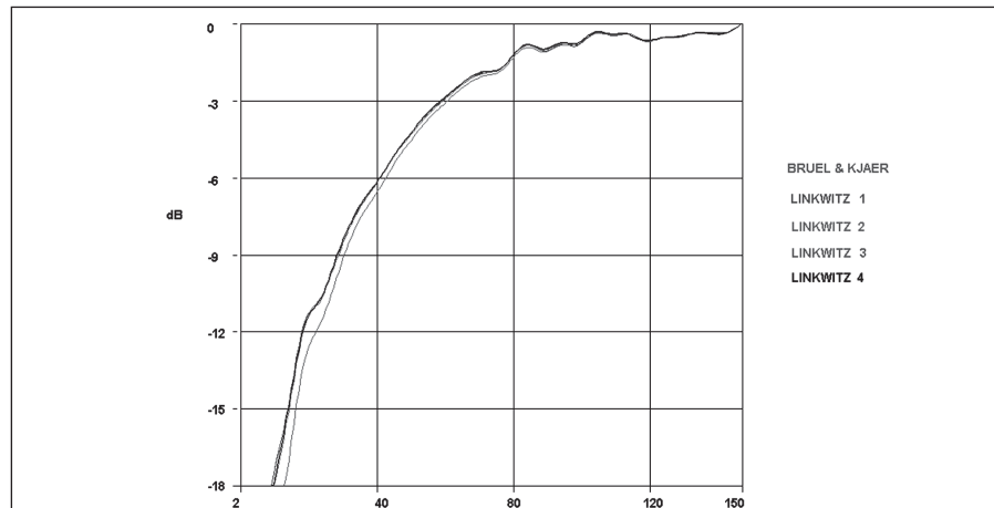
Figure 5: The low frequency response of the acoustic source as measured by the B&K mike and the modified Panasonic mikes.
