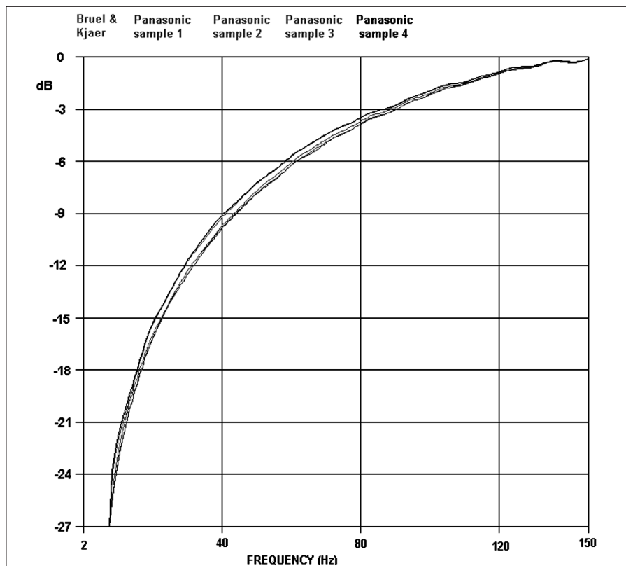
Figure 2: The low frequency response of the acoustic source as measured by the B&K mike and the standard Panasonic mikes.
