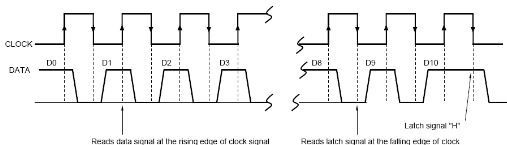
FIGURE 2-2 TIMING DIAGRAM
