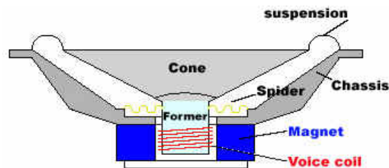
"Typical" Driver Construction
