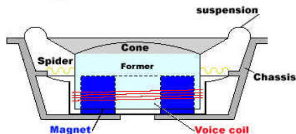
Dynaudio Driver Construction
