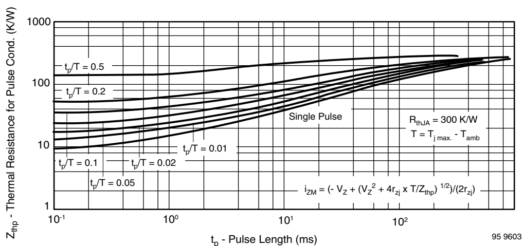
Fig. 11 - Thermal Response
