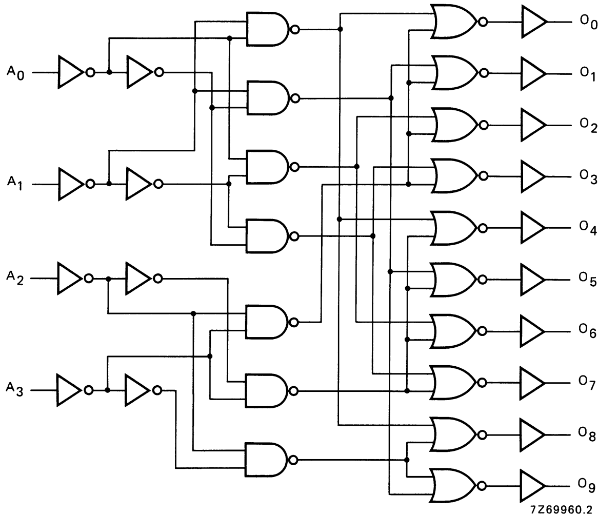
Fig.3 Logic diagram.
