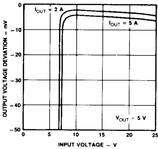
Line Regulation
