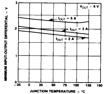
Dropout Voltage
