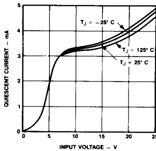
Quiescent Current
