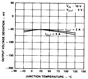
Output Voltage Deviation vs Junction Temperature
