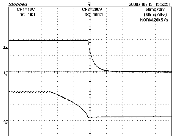
Figure 21 - Shut-down, No-load, 85 V_{AC} V_{OUT} & V_{C7} (10 & 100V/div, 50ms/div)
