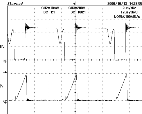
Figure 16 - V_{DRAIN} & I_{DRAIN} (100 V & 1 A /div) at 70 Watt load, 265VAC input. (2 \mu S/div)
