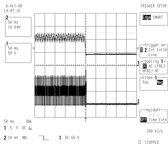
Figure 26 - Shut-down, 5.25 \Omega load, 85 V_{AC} V_{C7} & I_{DRAIN} (50 V & 1A/div, 50ms/div)
