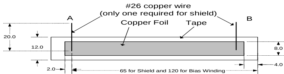
Figure 1-A (Top View before folding tape)
