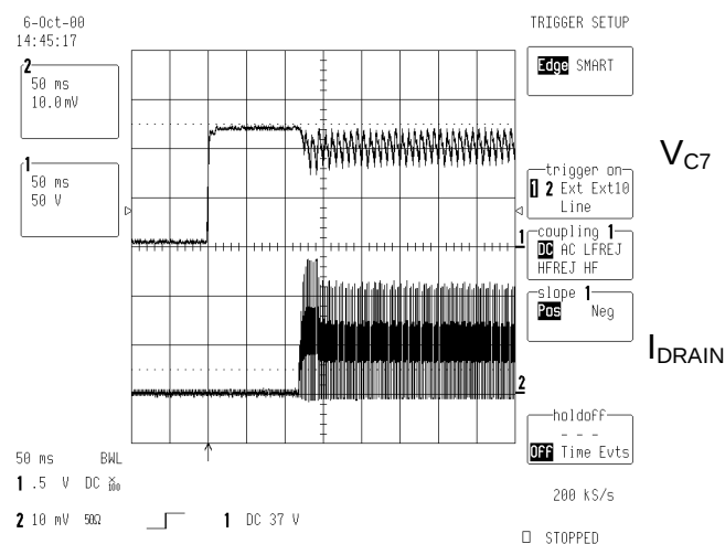
Figure 25 - Start-up, 5.25 \Omega load, 85 V_{AC} V_{C7} & I_{DRAIN} (50 V & 1A/div, 50ms/div)
