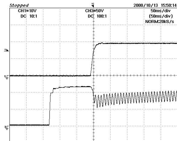
Figure 17 - Start-up, 5.25 \Omega load, 85 V AC V_{OUT} & V_{C7} (10 & 100 V/div, 50ms/div)
