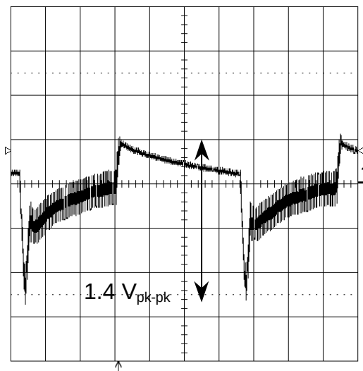
Figure 30 - Transient Response 265 V AC 50 Hz, I OUT : 0 A to 1.83 A V OUT (200 mV, 5ms/div)
