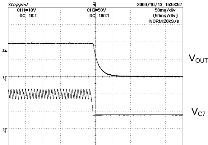
Figure 20 - Shut-down, 5.25 \Omega load, 85 V_{AC} V_{OUT} & V_{C7} (10 & 100V/div, 50ms/div)
