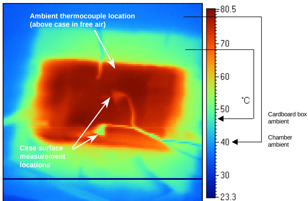
Figure 14 - Thermal image of case at 45°C ambient, 70 W output and 90 V AC input
