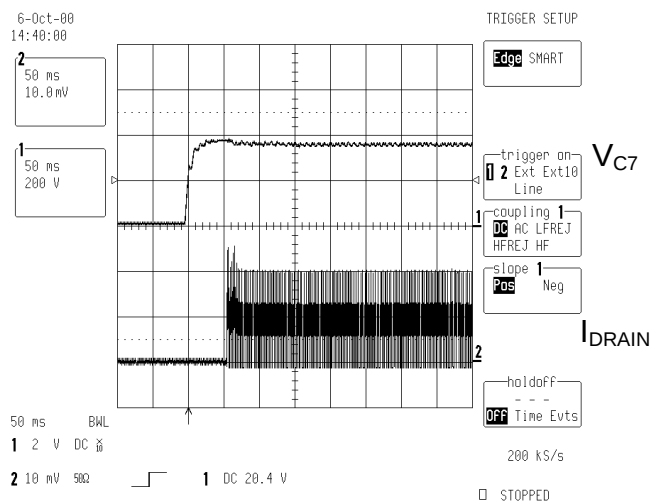
Figure 23 - Start-up, 5.25 \Omega load, 265 V_{AC} V_{C7} & I_{DRAIN} (200 V & 1A/div, 50ms/div)
