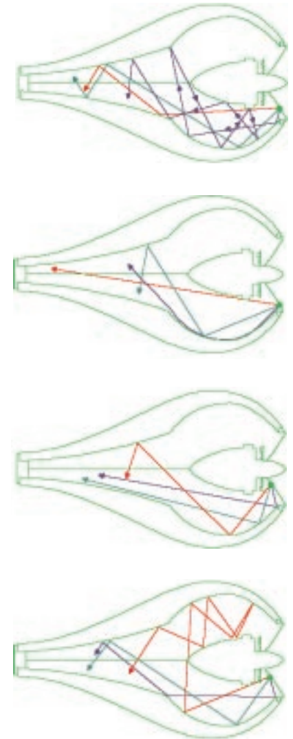
15 Some simplified vector representations of the radiation from a diaphragm visualised as a number of omnidirectional high frequency virtual point sources. This shows how the sphere/tube combination minimises reflections back to the diaphragm. Note: lossy wadding is placed in sphere and diaphragm's rear suspension disperses/absorbs coil area reflections
