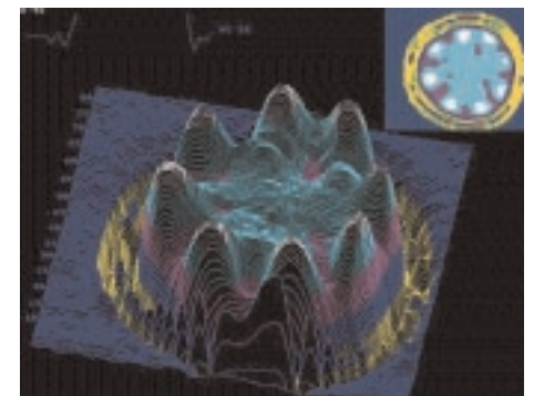
AV-3 Phase sensitive whole cone plot. Peaks and dips cancel out, surround sound resonance does not.
