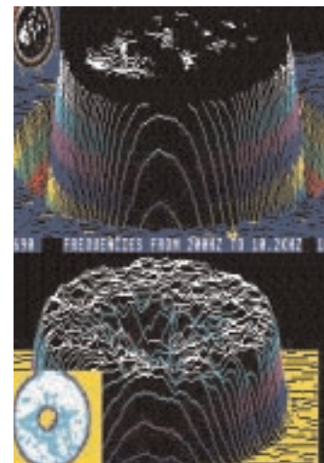
b The Kevlar® Driver's edges begin to give way above 3kHz
