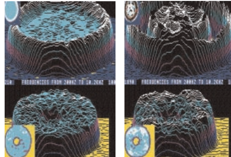
A1-3 Kevlar® and Plastic Drivers Compared (Frequency Plot) a The Plastic driver shows many resonances all through the band and beyond
