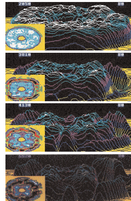
AV-2 Whole Cone Single Frequency Plots Top Picture at Low Frequency, Bottom at high Frequency Note: 4-way symmetry and smoothly reducing central area
