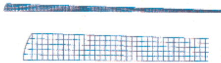
AIII-1 The Finite Element Model Upper – the entire model, Lower – close-up of the driver end
