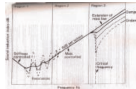
All-1 Mass Law + Stiffness + Coincidence
