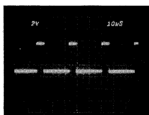
40 IC312 65, 66pin PLAY
