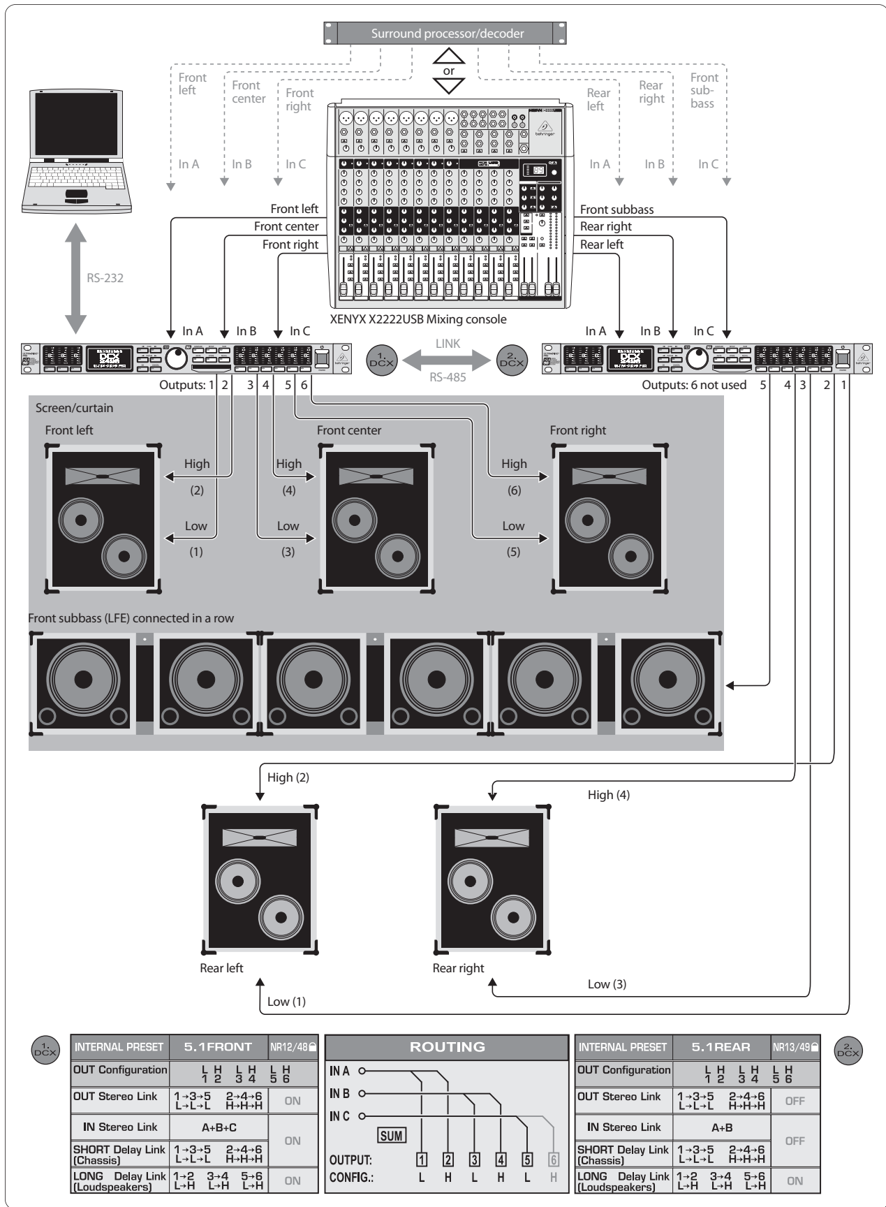
Afb. 6.12: Surround 5.1
