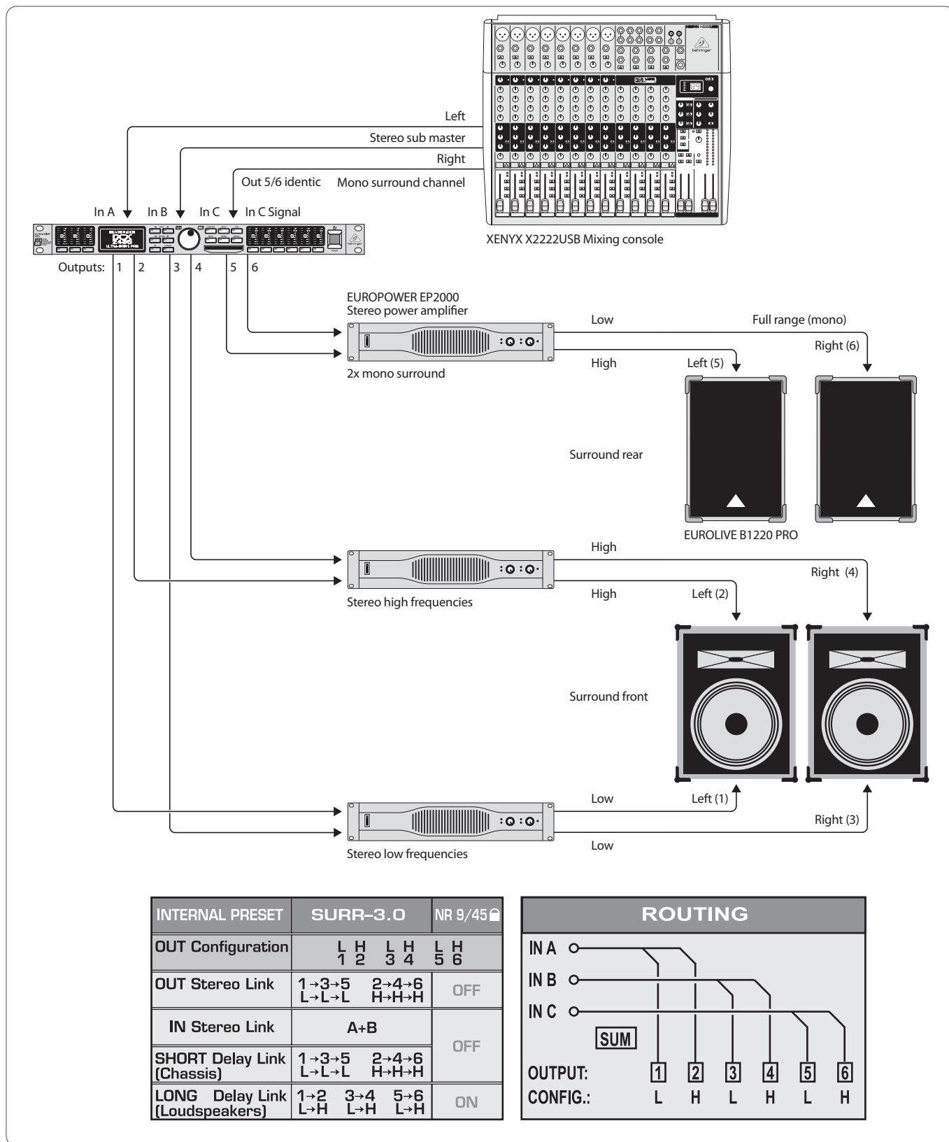
Afb. 6.9: Surround 3.0
