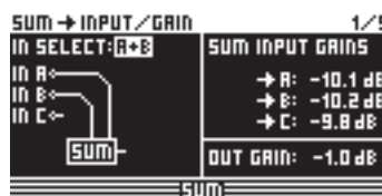
Afb. 4.37: Sum → Input/Gain
